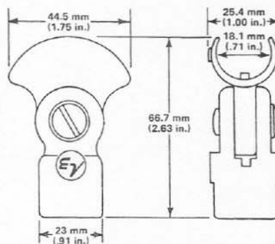
FIGURE 2 - 312 Dimensions
