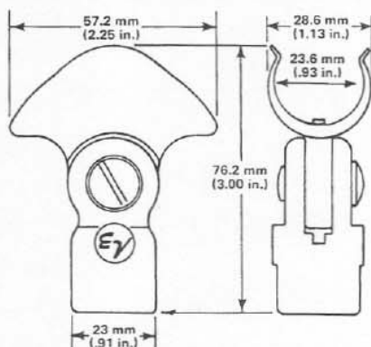
FIGURE 1 - 301 Dimensions
